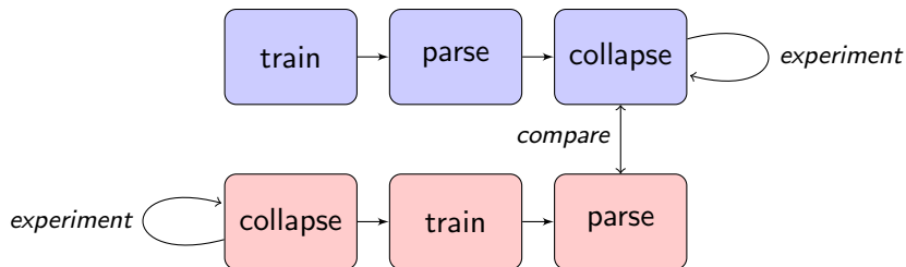
Figure : Pipeline
